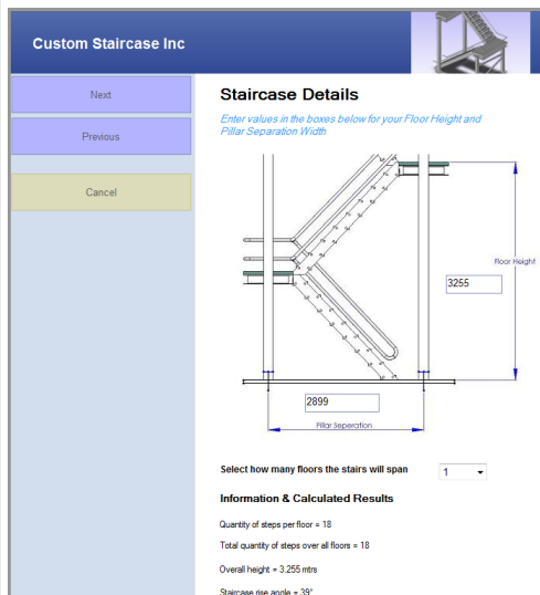
DriveWorks Form in Internet Explorer
